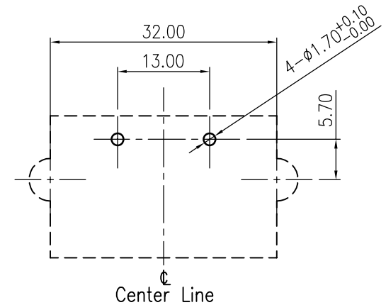
P.C.B Layout Dimension (Tolerance:±0.1) (Recommend min.Dimension)(bottom view)
