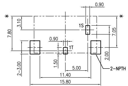
PCB Layout Dimension (Tolerance: ±0.05) (Recommend min. Dimension)(Bottom View)
