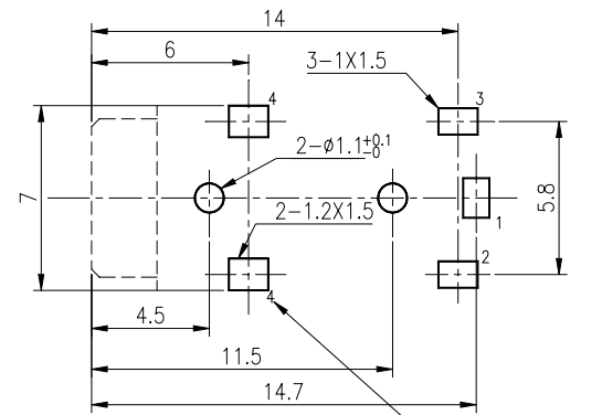
HOLE LAYOUT (BOTTOM VIEW) (TOLERANCE :±0.1) (t=1)
