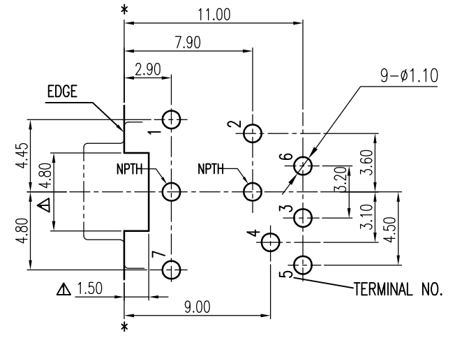
P.C.B Layout Dimension(Tolerance:±0.1) (Recommend min. Dimension)(Bottom View)
