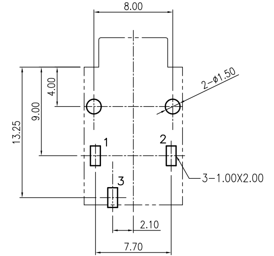
PCB Layout Dimension (Tolerance: \pm 0.10 ) (Recommend min. Dimension)(Bottom View)
