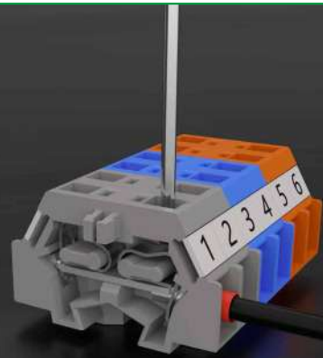
Spring Cage Type Terminal Block
