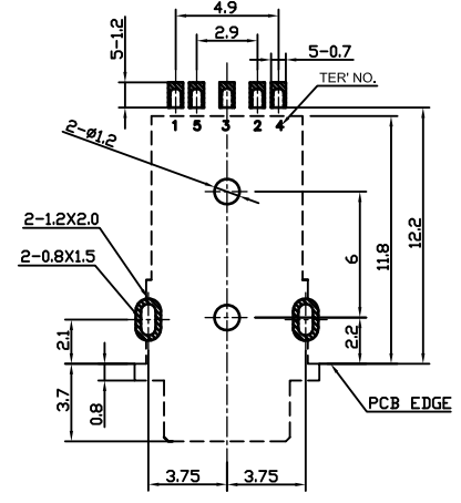
RECOMMENDED PCB MOUNTING HOLES (TOP VIEW)(tolerance±0.05)
